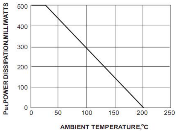
Admissible power dissipation versus ambient temperature
