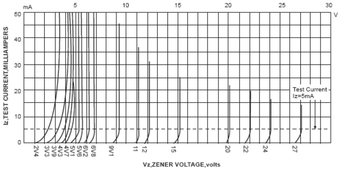
Breakdown characteristics
