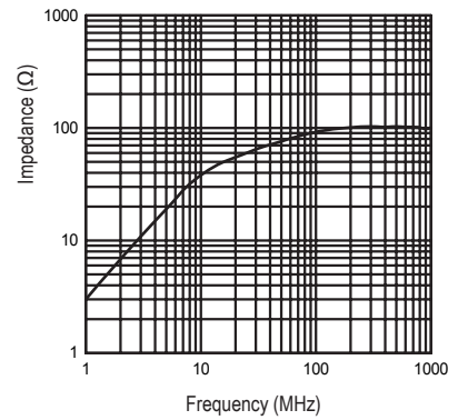
Typical Z vs Frequency
